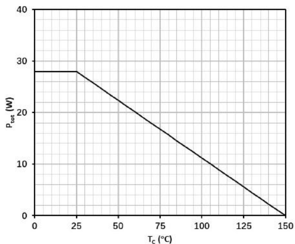
Figure 14 Power dissipation
