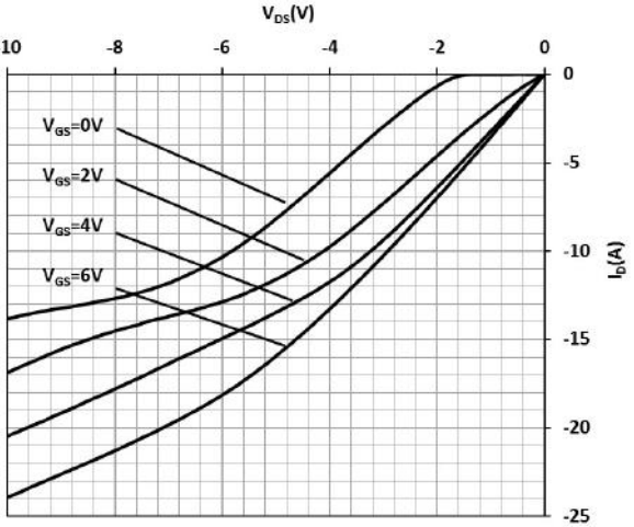
Figure 8 Typ. channel reverse characteristics
